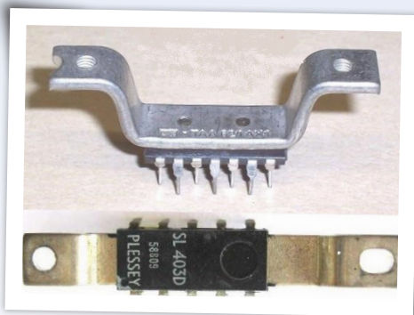
Figure 6: Audio amplifiers with heatsink. A quad-in-line TAA621 (top), and a Plessey SL403D (bottom).
