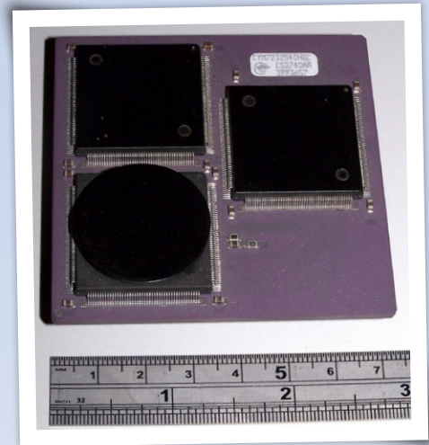
Figure 7: Early 1990s DRAM accelerator IC.
