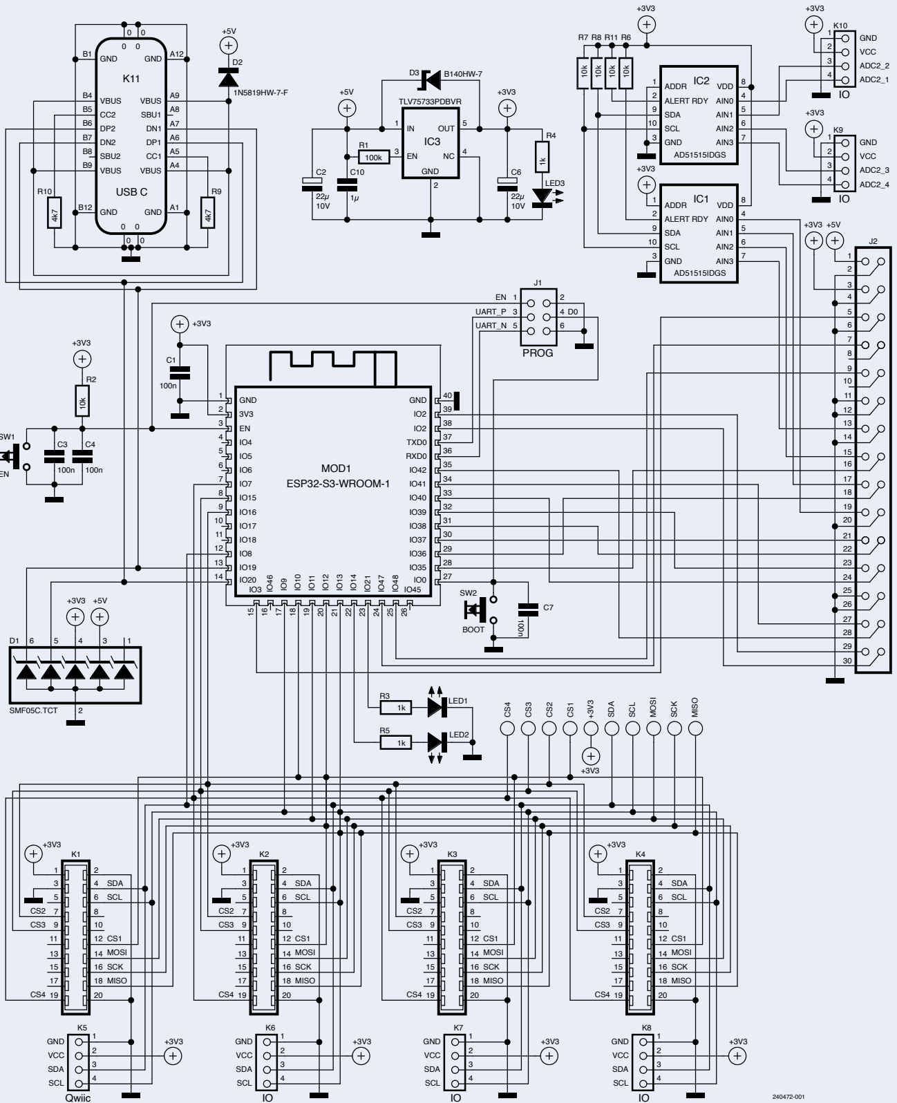
Figure 2: Schematic diagram of the project.
